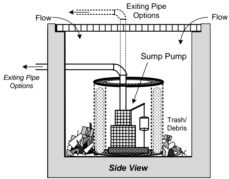
TRITON – CSPF (Cartridge Sump Pump Filter) SERIES FILTER By REM Inc. (888.526.4736) www.remfilters.com
