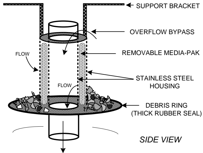
TRITON – MINI-GT'S (For Area Drains) SERIES FILTER By REM Inc. (888.526.4736) www.remfilters.com
