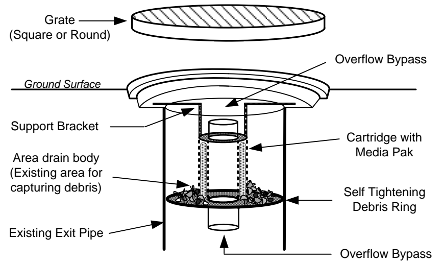
TRITON – MINI-GT'S (For Area Drains) SERIES FILTER By REM Inc. (888.526.4736) www.remfilters.com
