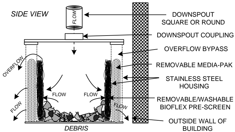
TRITON – 360 (Downspout) SERIES FILTER By REM Inc. (888.526.4736) www.remfilters.com
