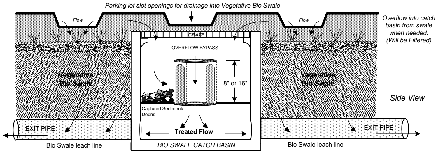
TRITON – TOP HAT (VEGETATIVE BIO SWALE) SERIES #4 FILTERS (For Bioretention Areas) By REM Inc. (888.526.4736) www.remfilters.com
