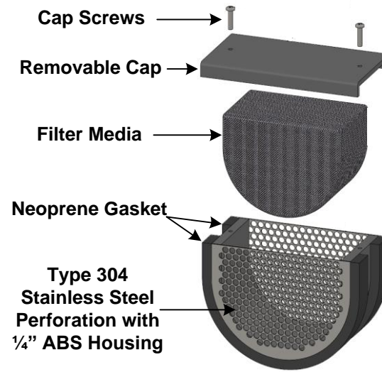
TRITON – TDAM TT2 SERIES FILTER By REM Inc. (888.526.4736) www.remfilters.com
