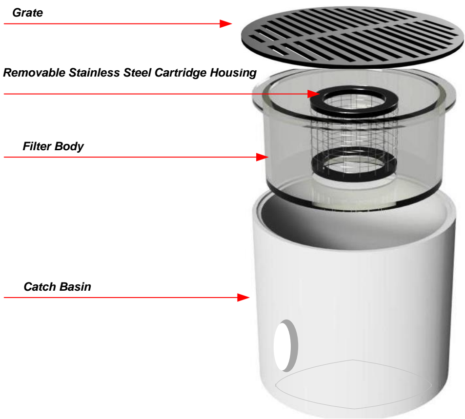
Round Catch Basin Shown
