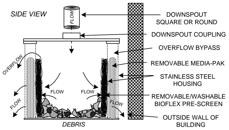
TRITON – 360 (Downspout) SERIES FILTER By REM Inc. (888.526.4736) www.remfilters.com
