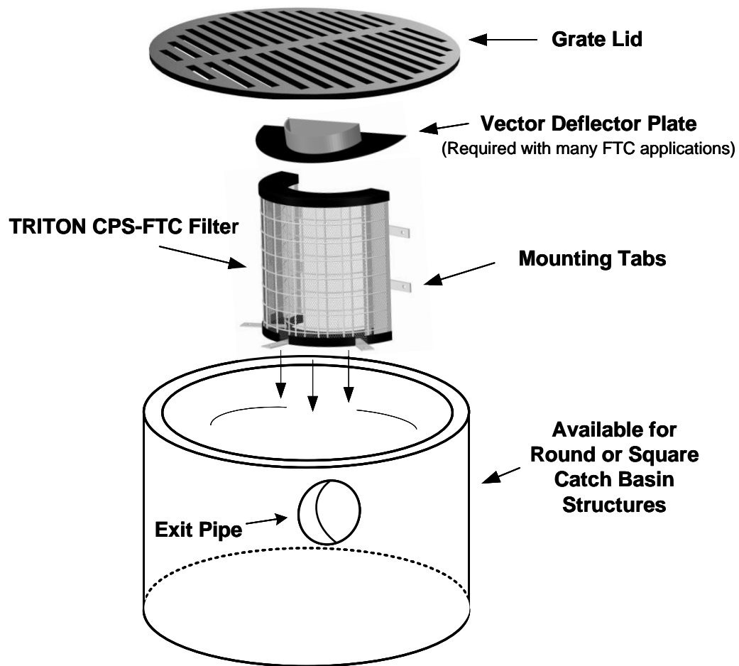
TRITON – CPS-FTC Series Crescent Pipe Screen Full Trash Capture Filter Series By REM Inc. (888.526.4736) www.remfilters.com
